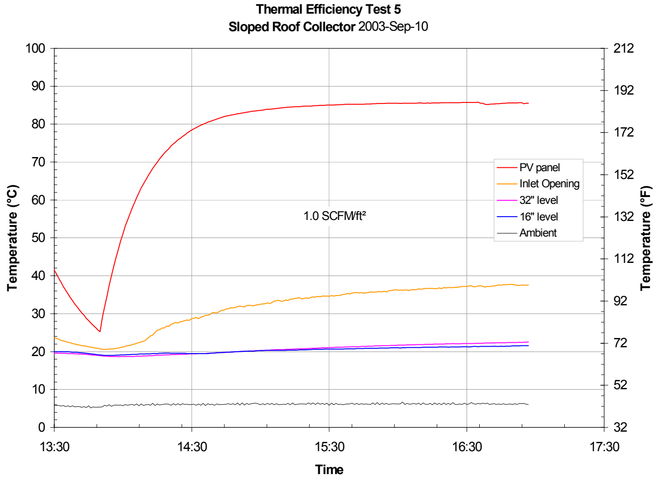
Figure 11. Air temperatures recorded during fifth thermal efficiency test.
