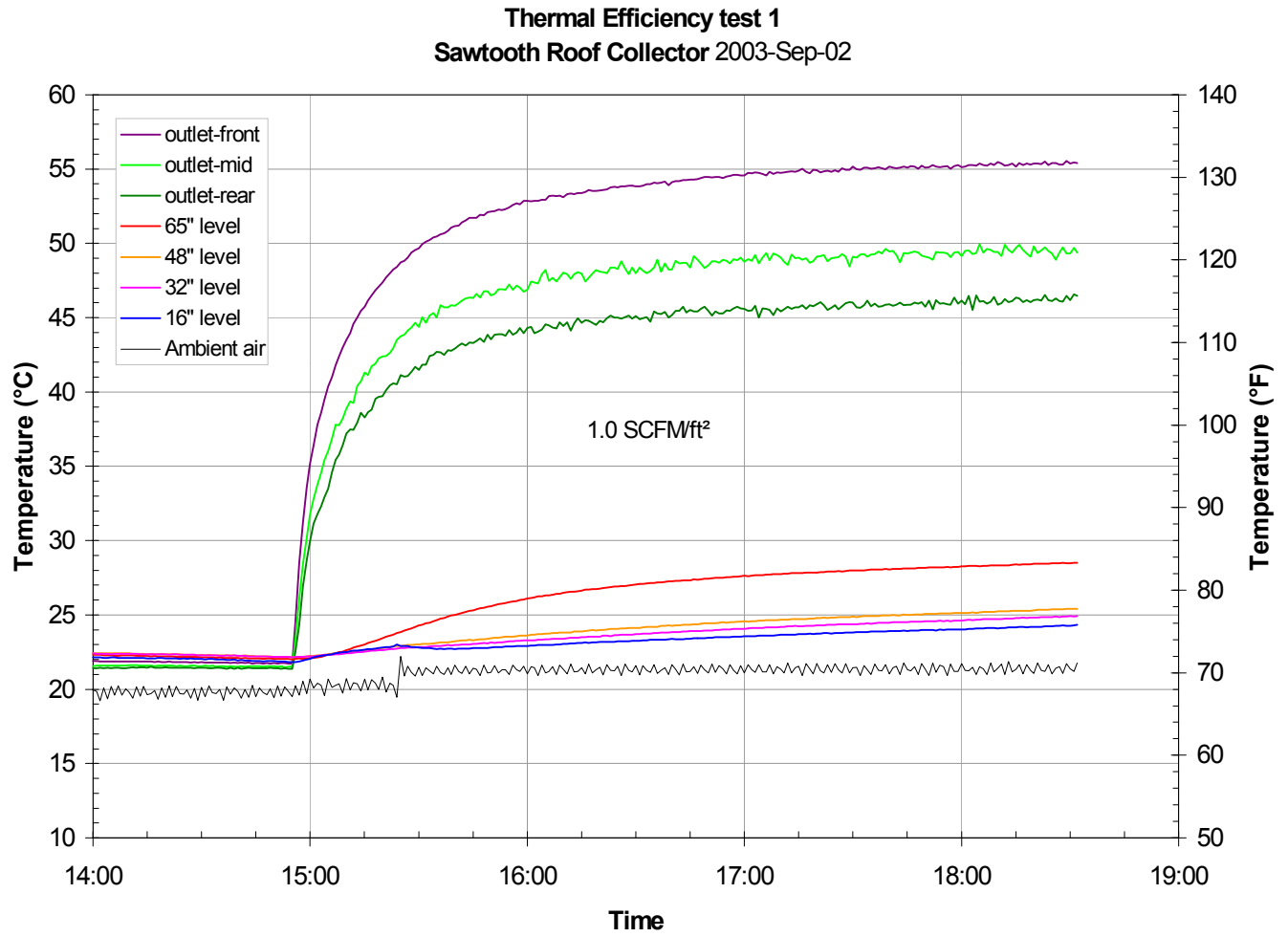
Figure 2. Air temperatures recorded during first thermal efficiency test.
