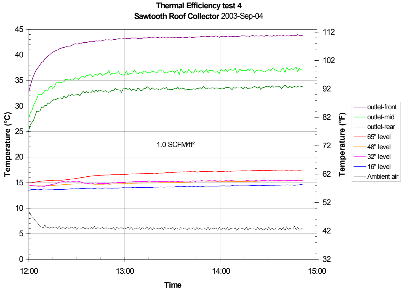
Figure 5. Air temperatures recorded during fourth thermal efficiency test.
