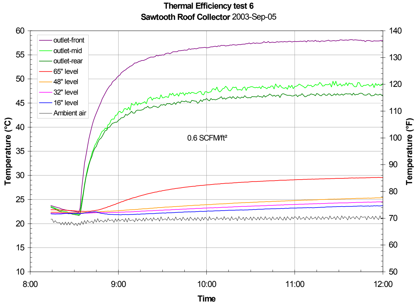
Figure 7. Air temperatures recorded during sixth thermal efficiency test.
