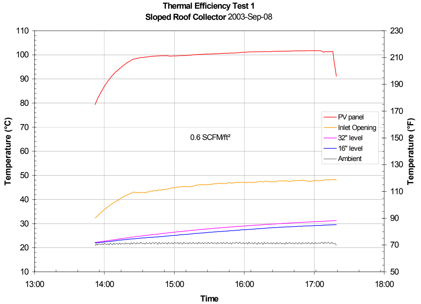
Figure 8. Air temperatures recorded during first thermal efficiency test of Sloped Roof collector.
