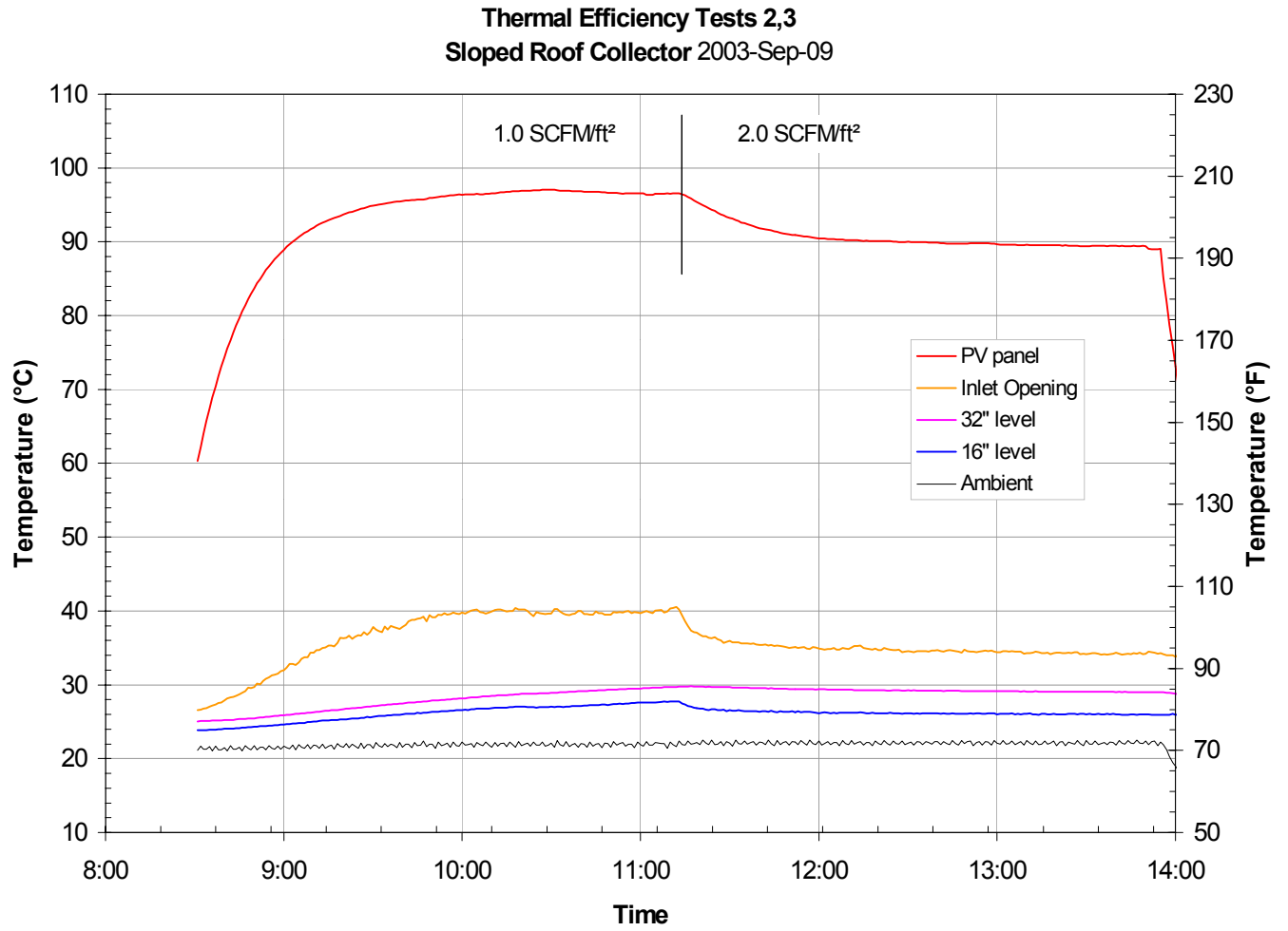
Figure 9. Air temperatures recorded during second and third thermal efficiency tests.
