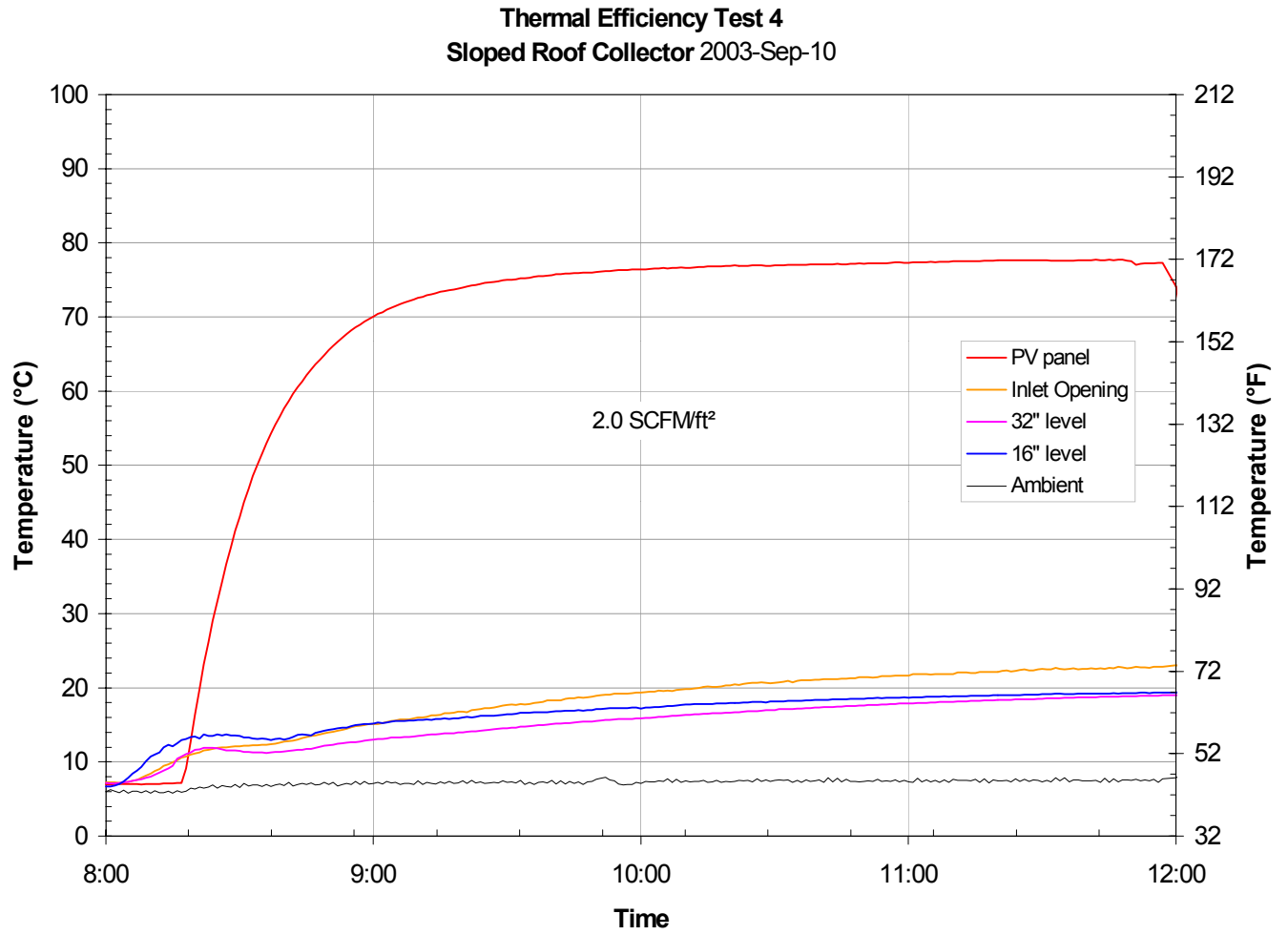
Figure 10. Air temperatures recorded during fourth thermal efficiency test.
