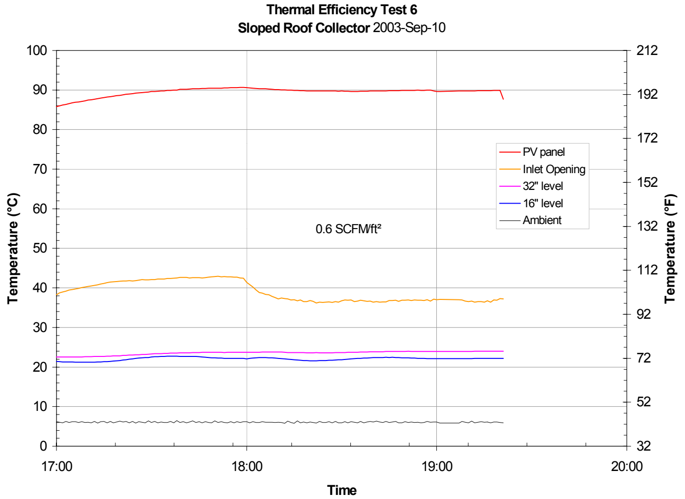
Figure 12. Air temperatures recorded during sixth thermal efficiency test.
