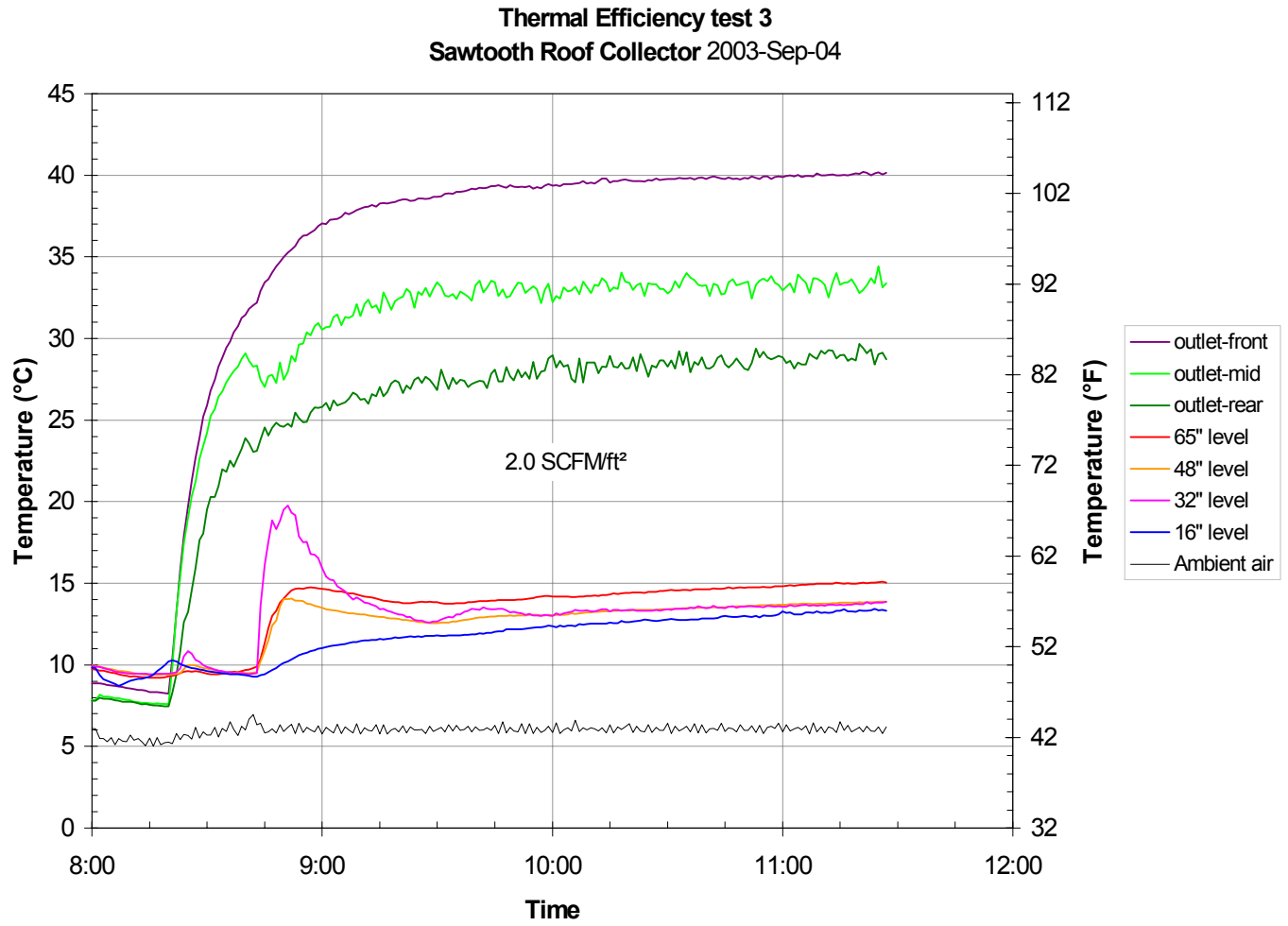
Figure 4. Air temperatures recorded during third thermal efficiency test.
