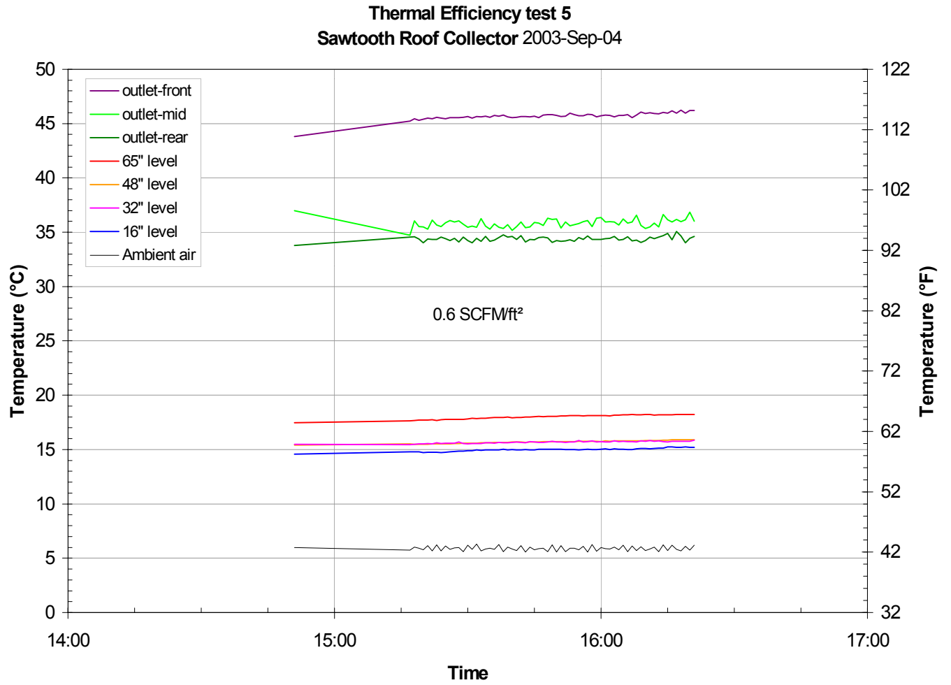
Figure 6. Air temperatures recorded during fifth thermal efficiency test.
